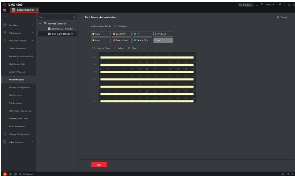
Figure 7-8 Set Authentication Modes for Card Readers
