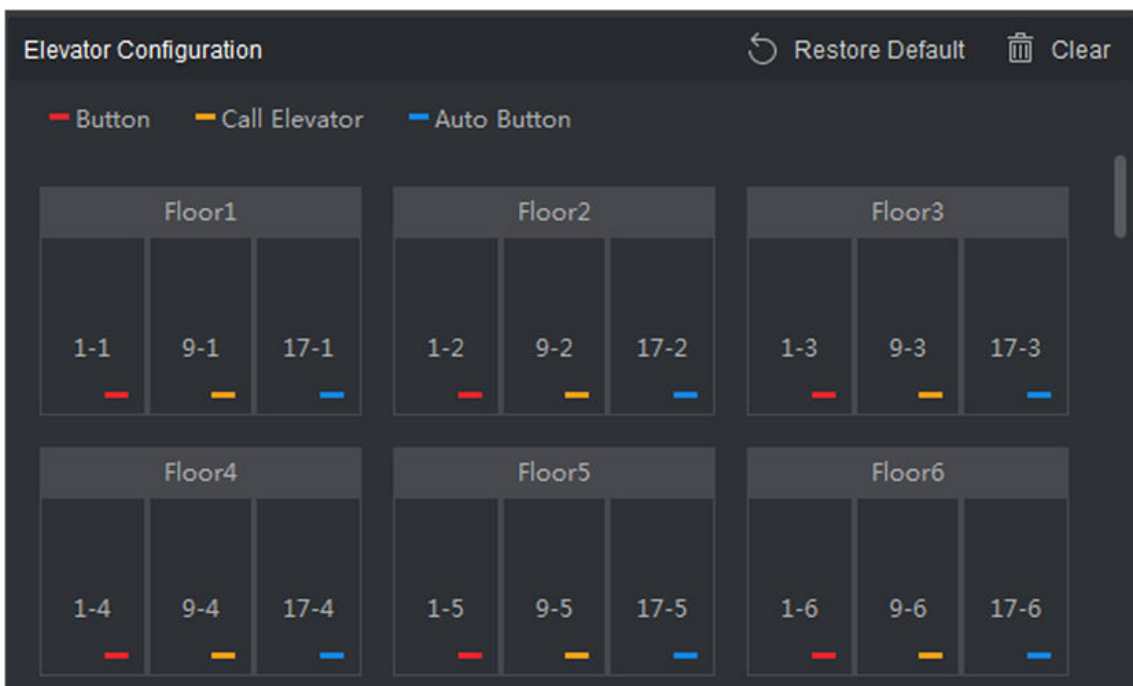
Figure 7-11 Relationship between Relay and Floor
