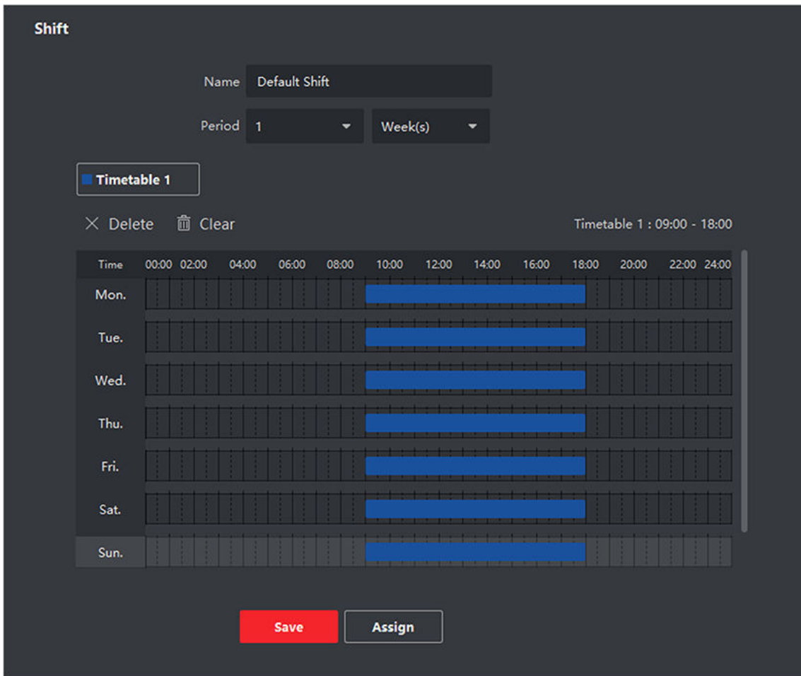
Figure 8-4 Add Shift
