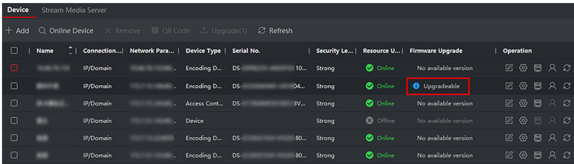
Figure 3-6 Firmware Upgrade
