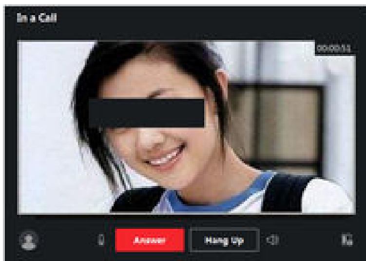
Figure 9-2 Incoming Call
