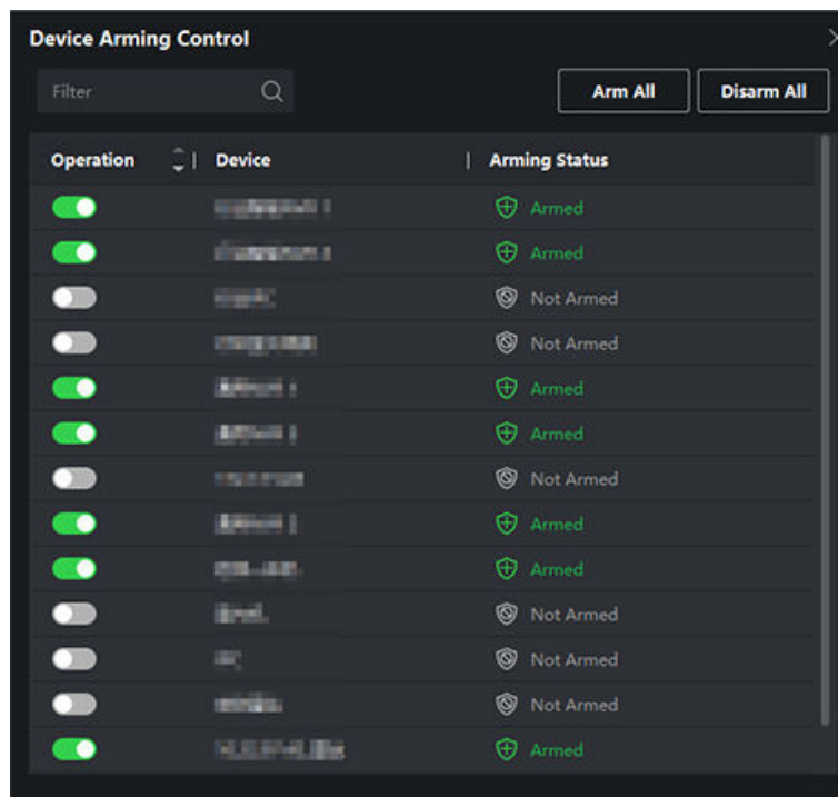
Figure 5-1 Arm Device
