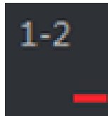
Figure 7-10 Relay
